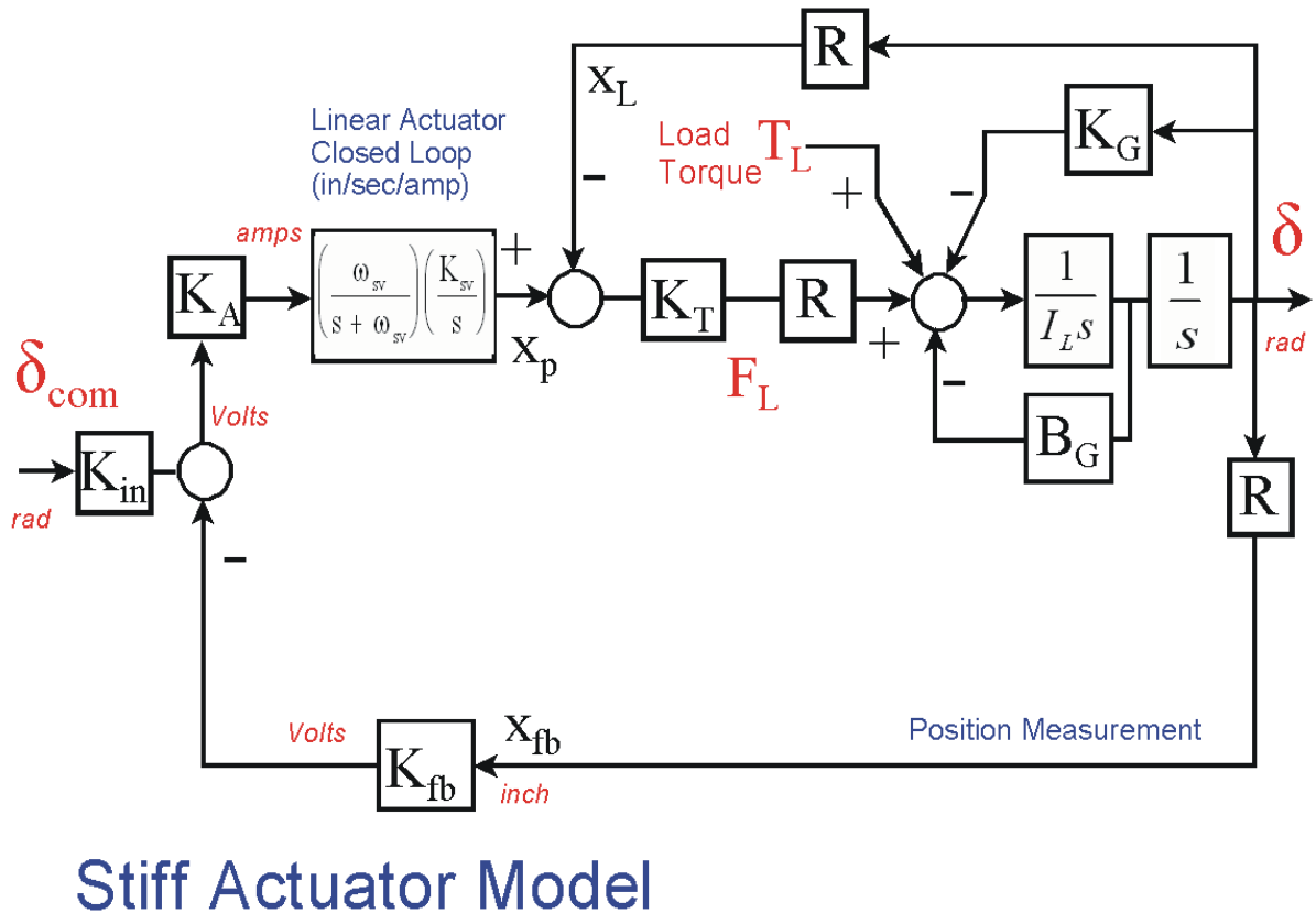
Figure (2.8.3) Stiff Actuator Model that includes only the Shaft Stiffness in ( K_T )
