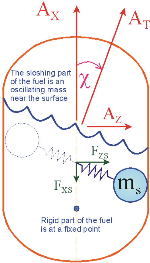
Figure (2.6.1) The slosh mass oscillates in a plane that is perpendicular to the average total acceleration and it creates oscillatory forces on the vehicle
