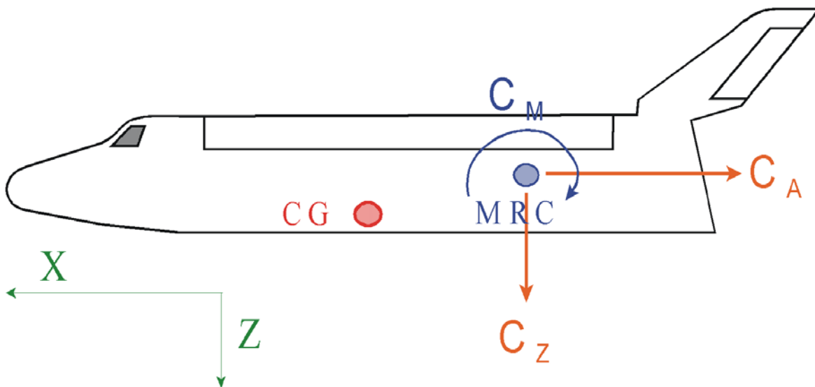
Figure 1.5.11 Pitch Moment Transformation from MRC to CG
