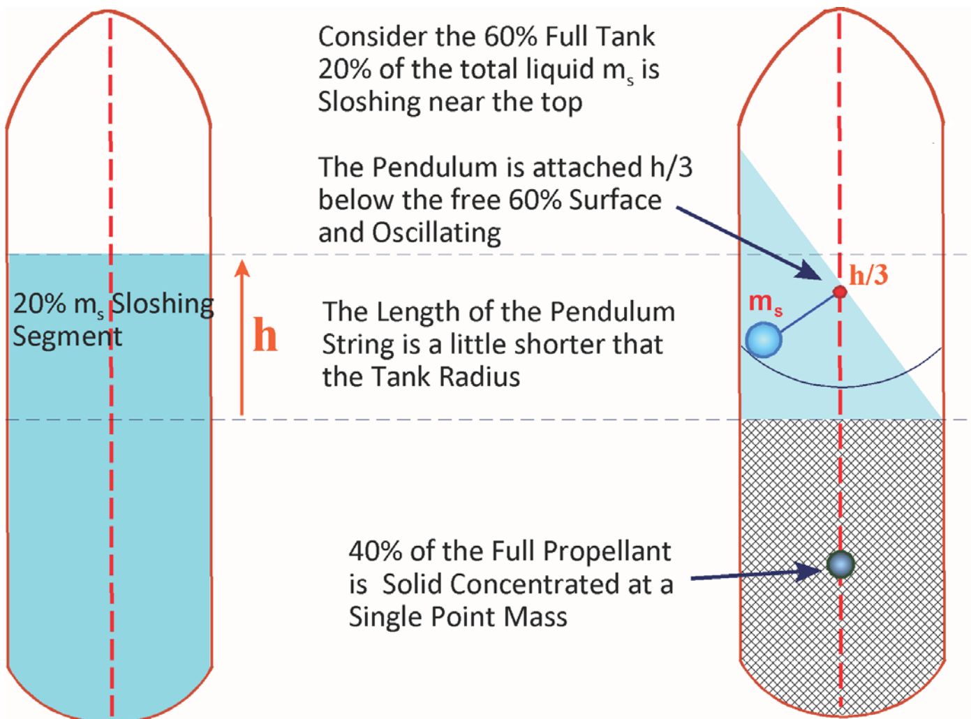
Figure 2.6.9 Pendulum Slosh Model
